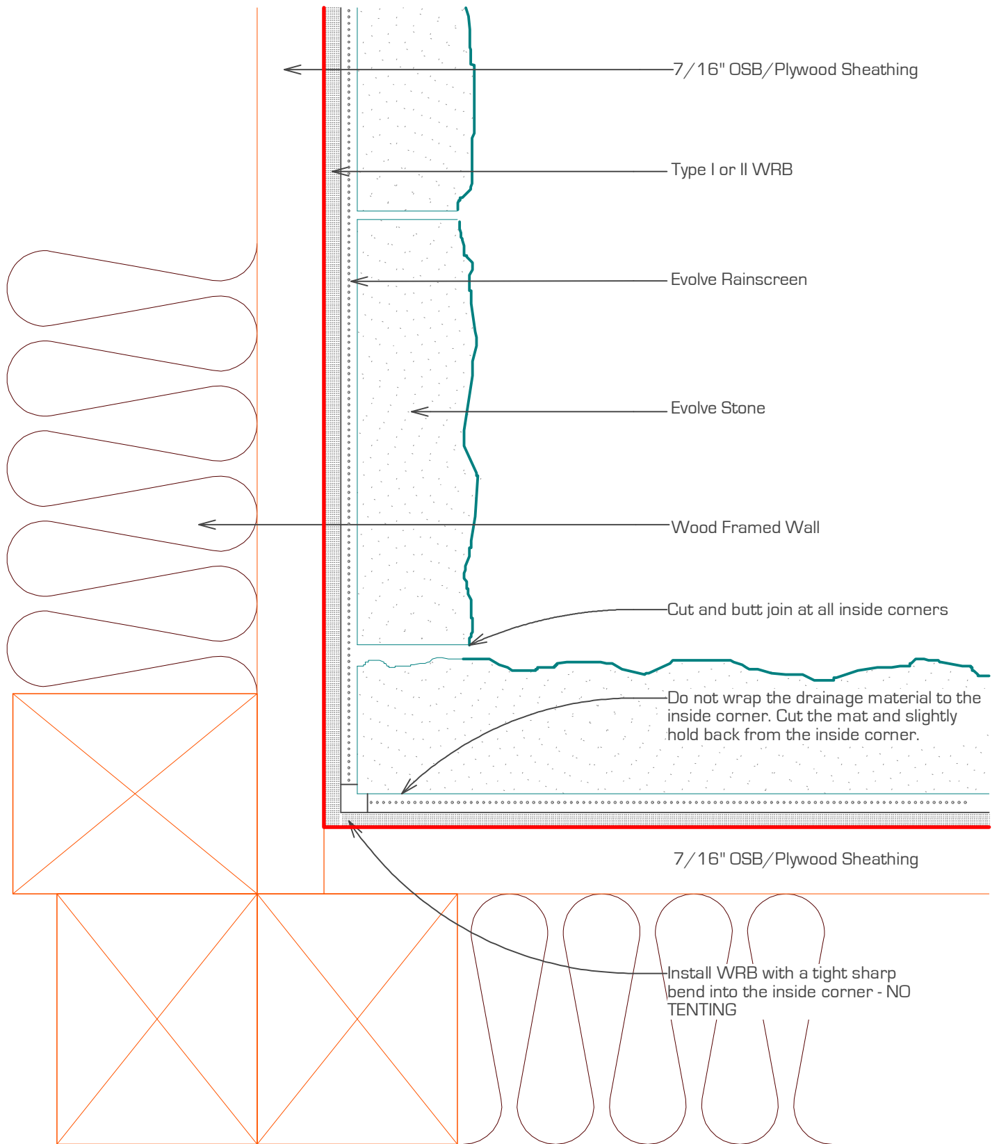
DETAIL #3
