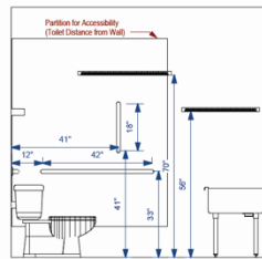
② Bathroom Elevation - Side Wall 1/2" = 1'-0"
