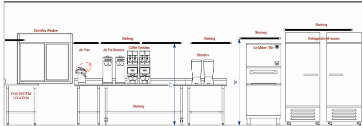
③ Interior Elevation - Facing DT 1/2" = 1'-0"
