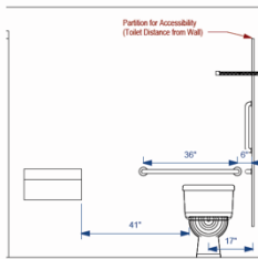
① Bathroom Elevation - Rear Wall 1/2" = 1'-0"
